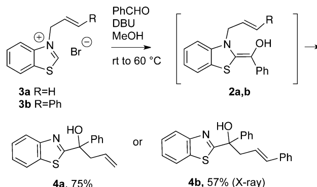
Scheme 2. [3,3] and [1,3] Rearrangements of N -allyl-substituted Breslow intermediates. [28] DBU = 1,8-diazabicyclo[5.4.0]undec-7-ene.
